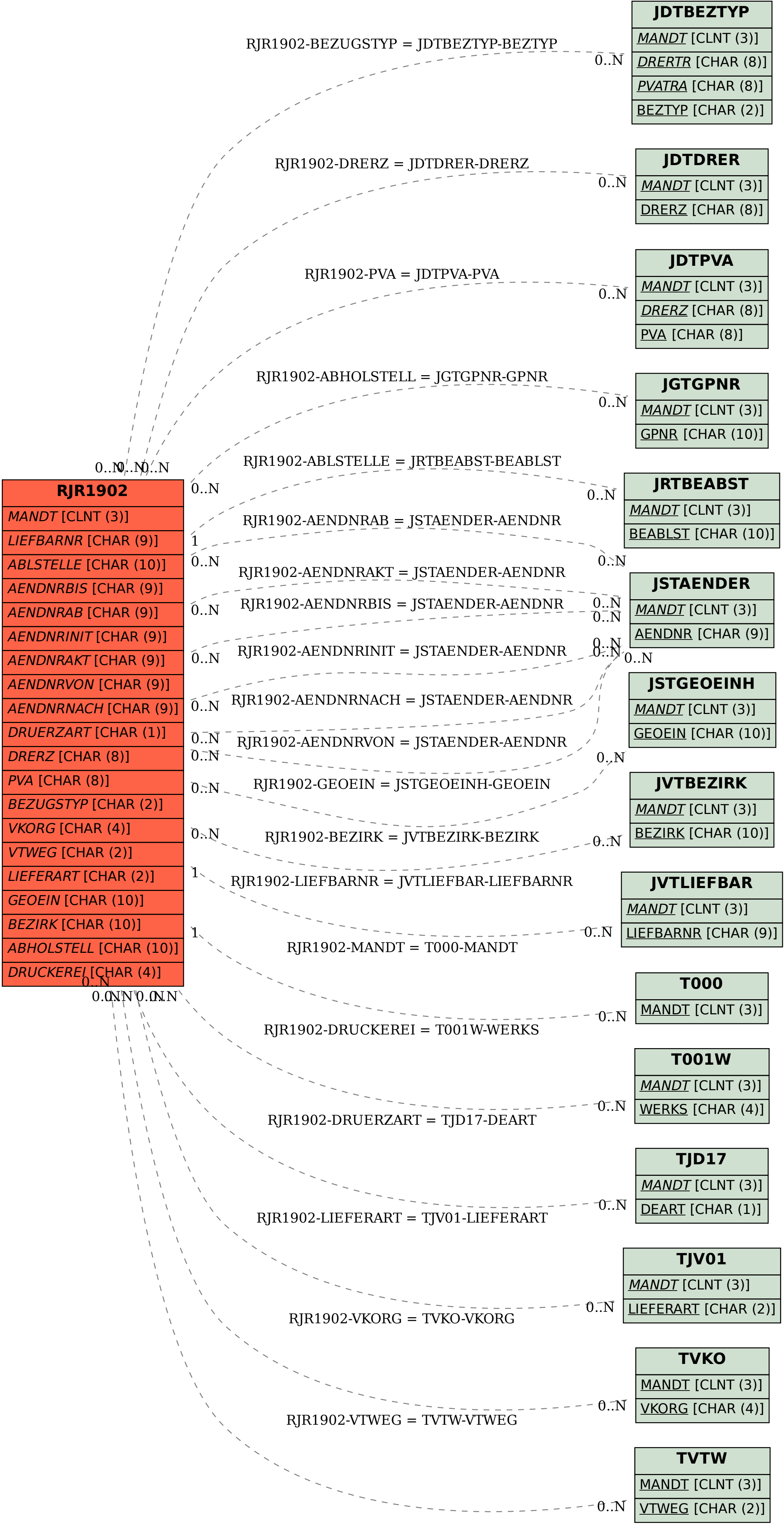
SAP ABAP table RJR1902 {IS-M/SD: Screen Display for Replacing Unloading Points TC}
