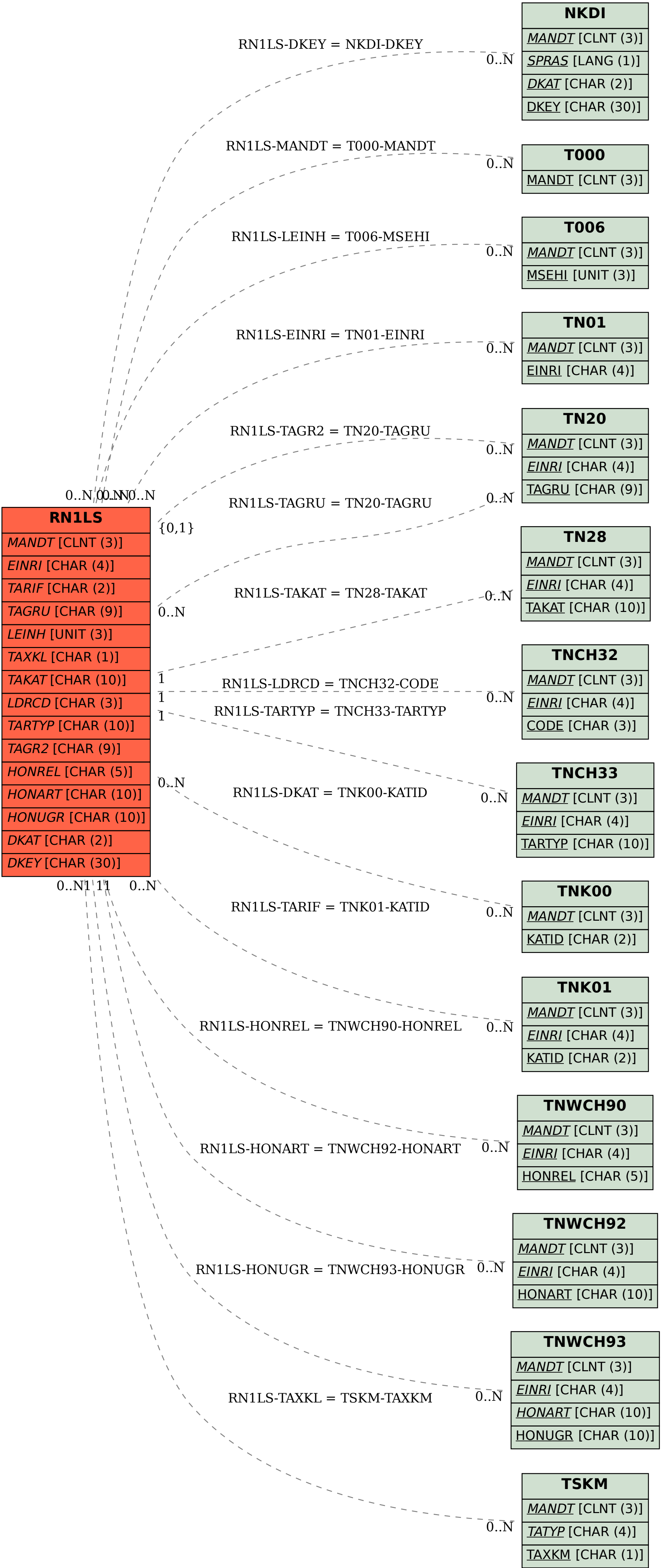
SAP ABAP table RN1LS {IS-H*MED: Structure for the ISHMED_NTPZ_HIERARCHIE}
