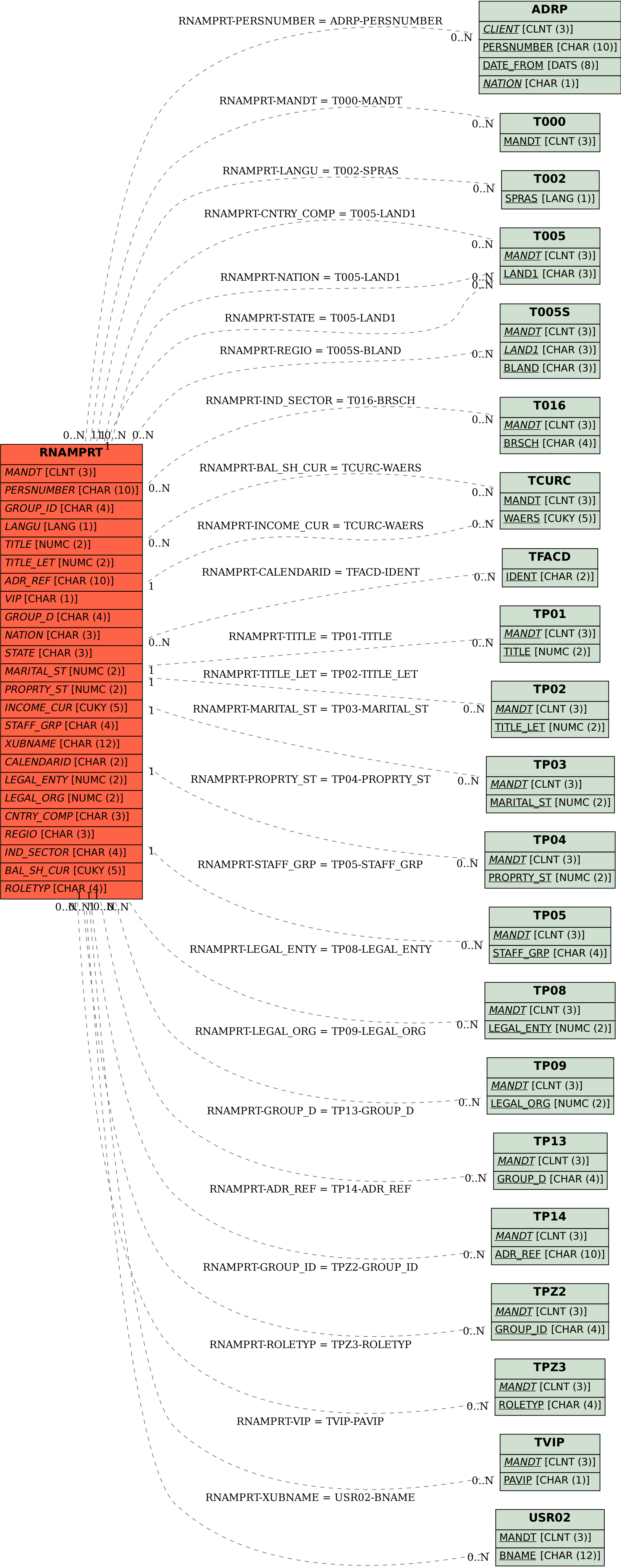
SAP ABAP table RNAMPRT {RE: Partner - Name and Additional Fields}
