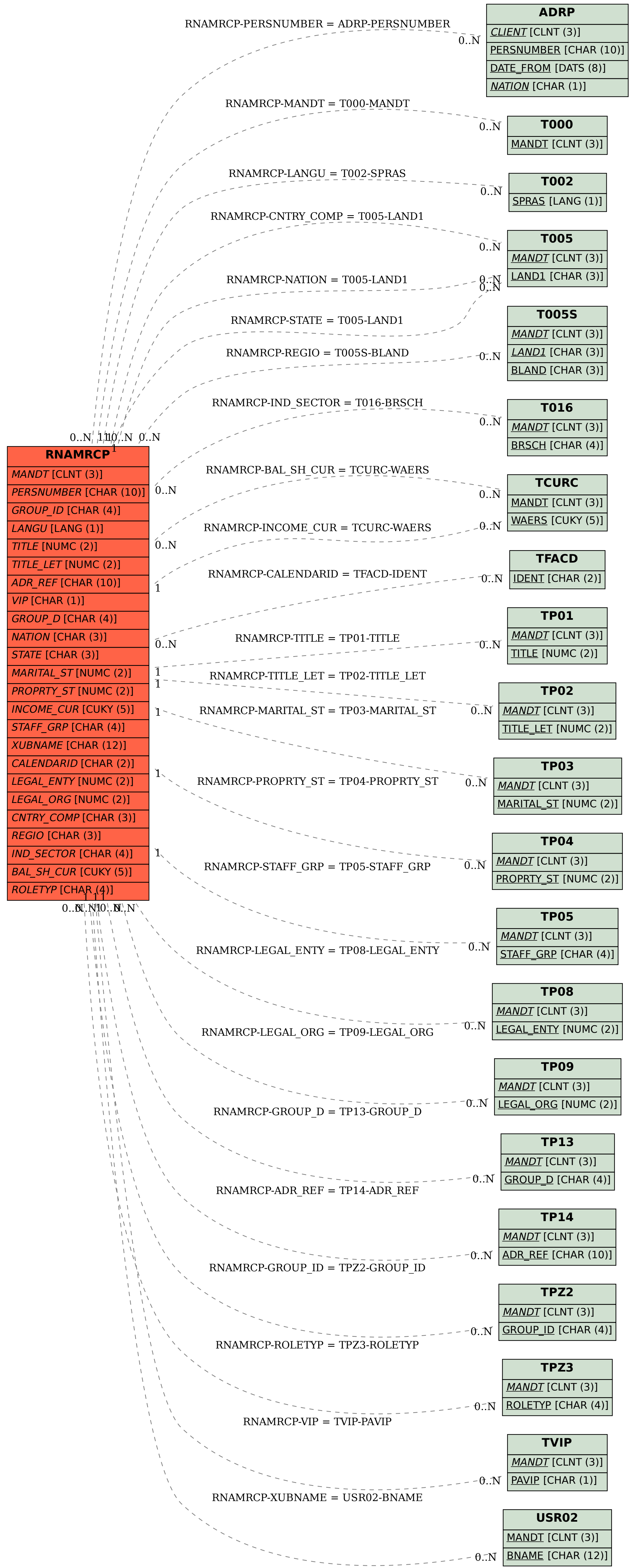
SAP ABAP table RNAMRCP {RE: Partner - Name of Letter Recipient and Addit.Fields}
