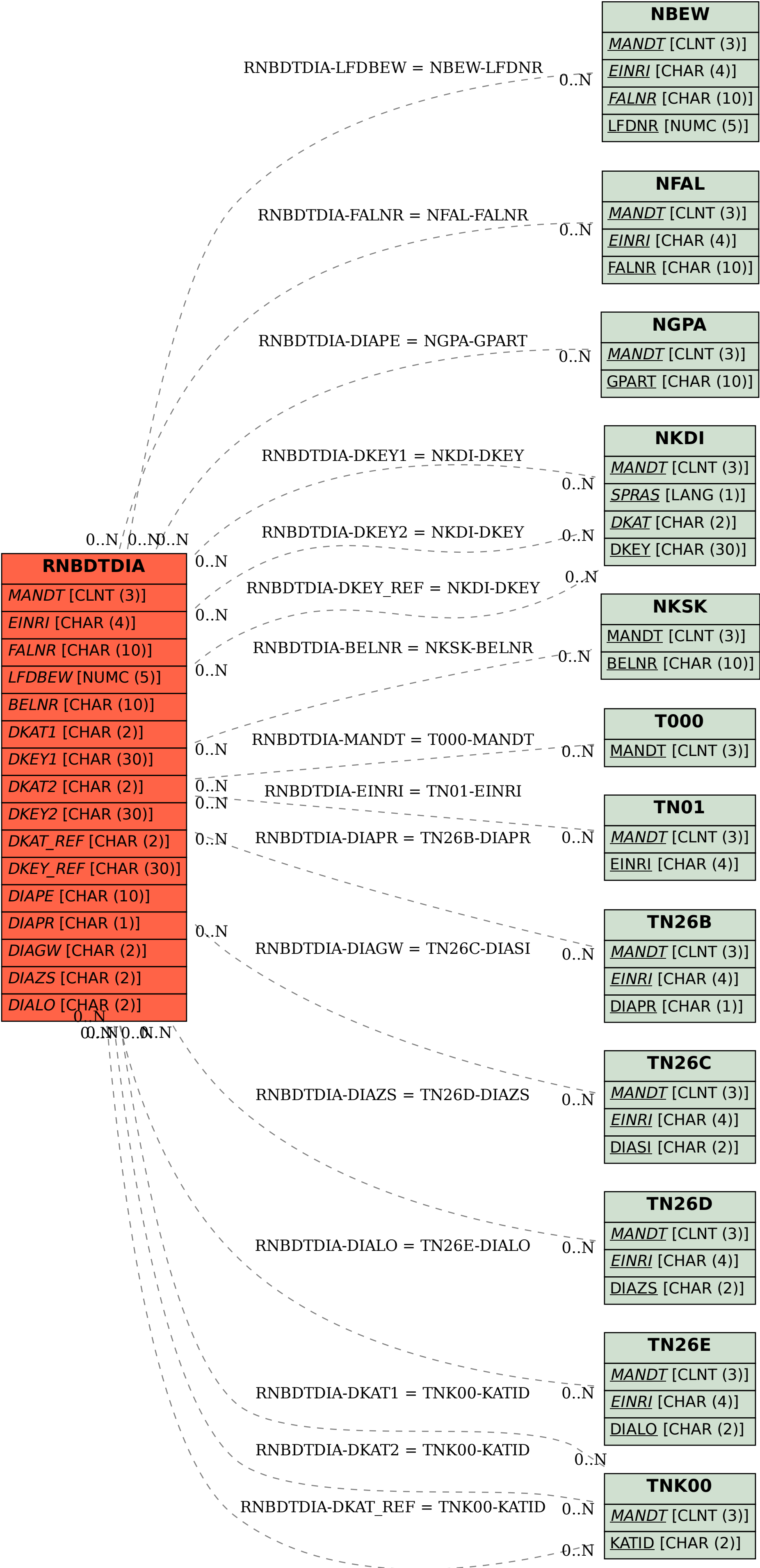
SAP ABAP table RNBDTDIA {IS-H (BDT format) : Structure for diagnoses}
