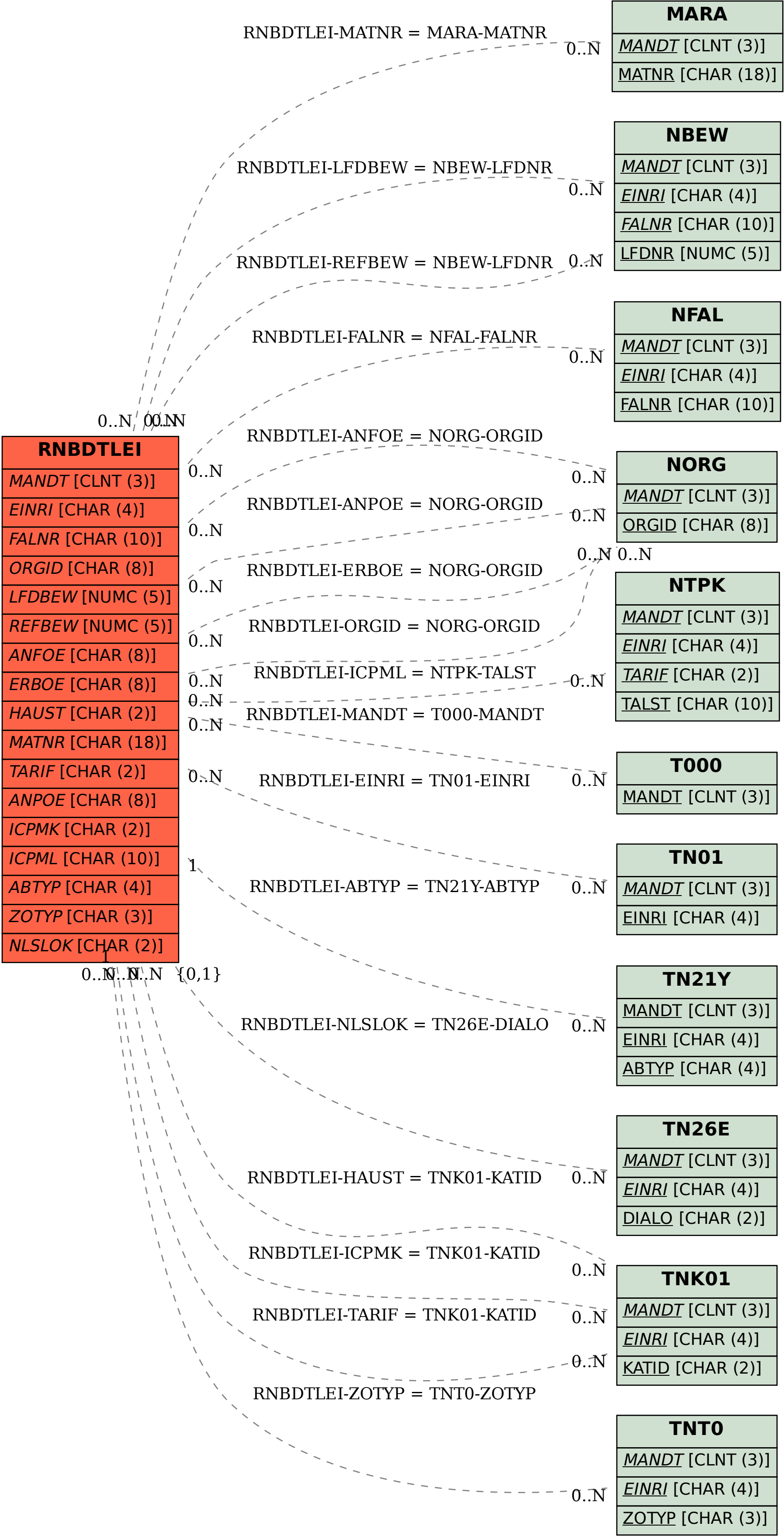
SAP ABAP table RNBDTLEI {IS-H (BDT format) : Structure for services}
