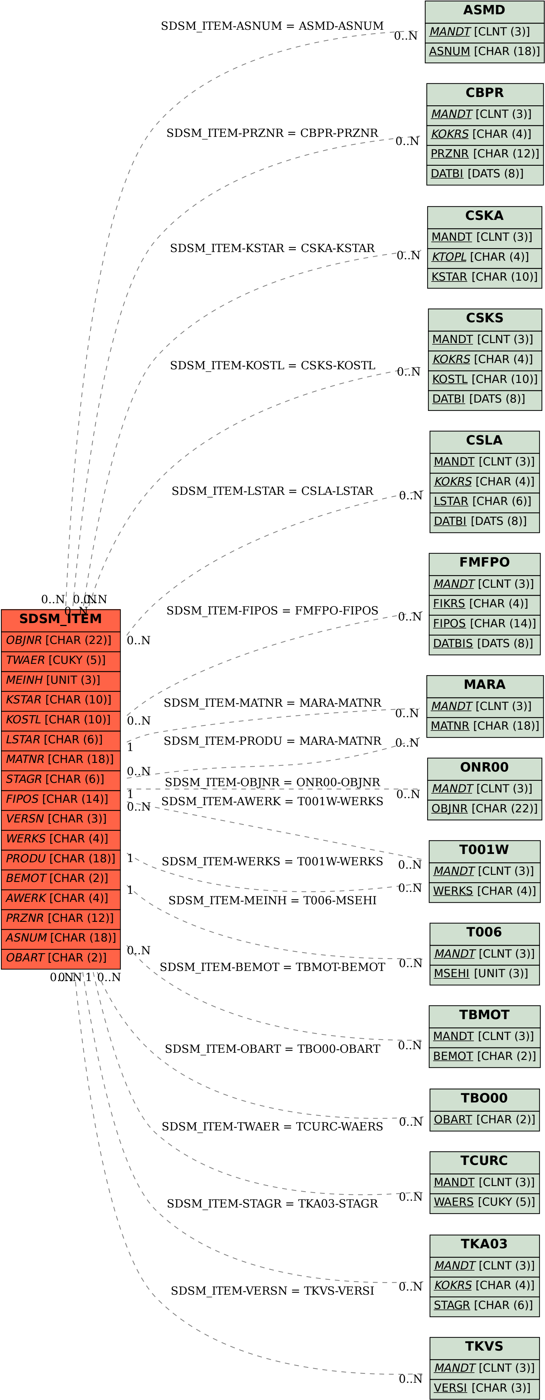
SAP ABAP table SDSM_ITEM {Item Data for Generating Sales Documents from Dynamic Items}
