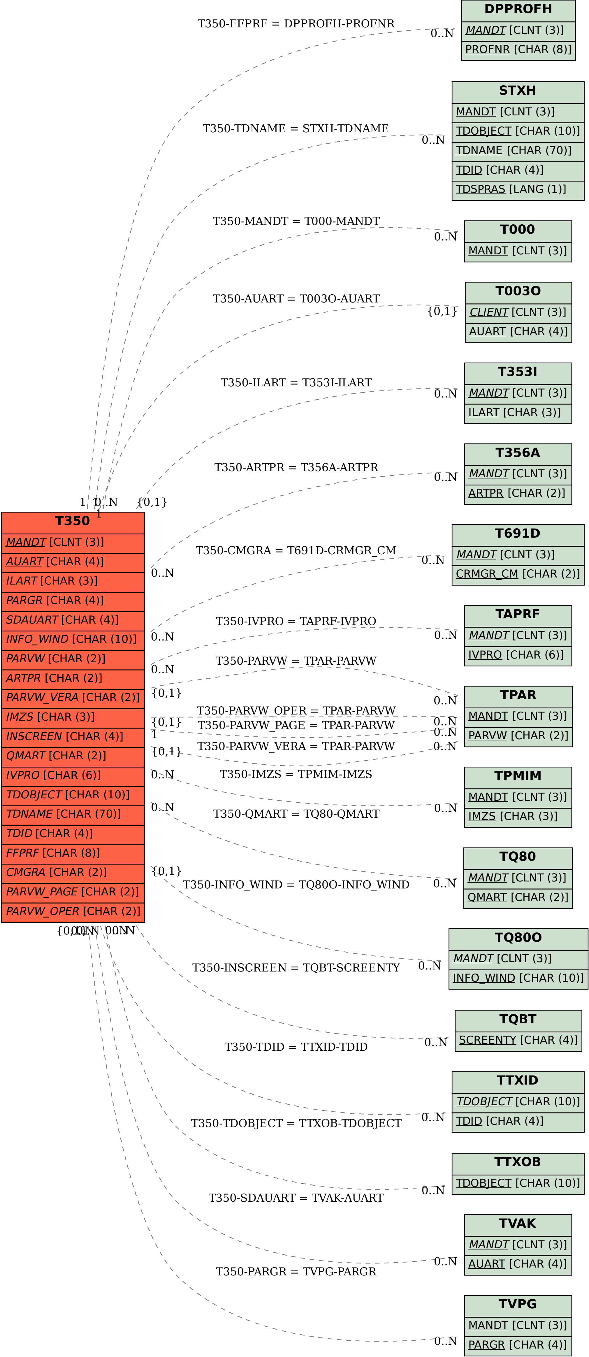
SAP ABAP table T350 {Maintenance Control Parameters: Client/Order Type}
