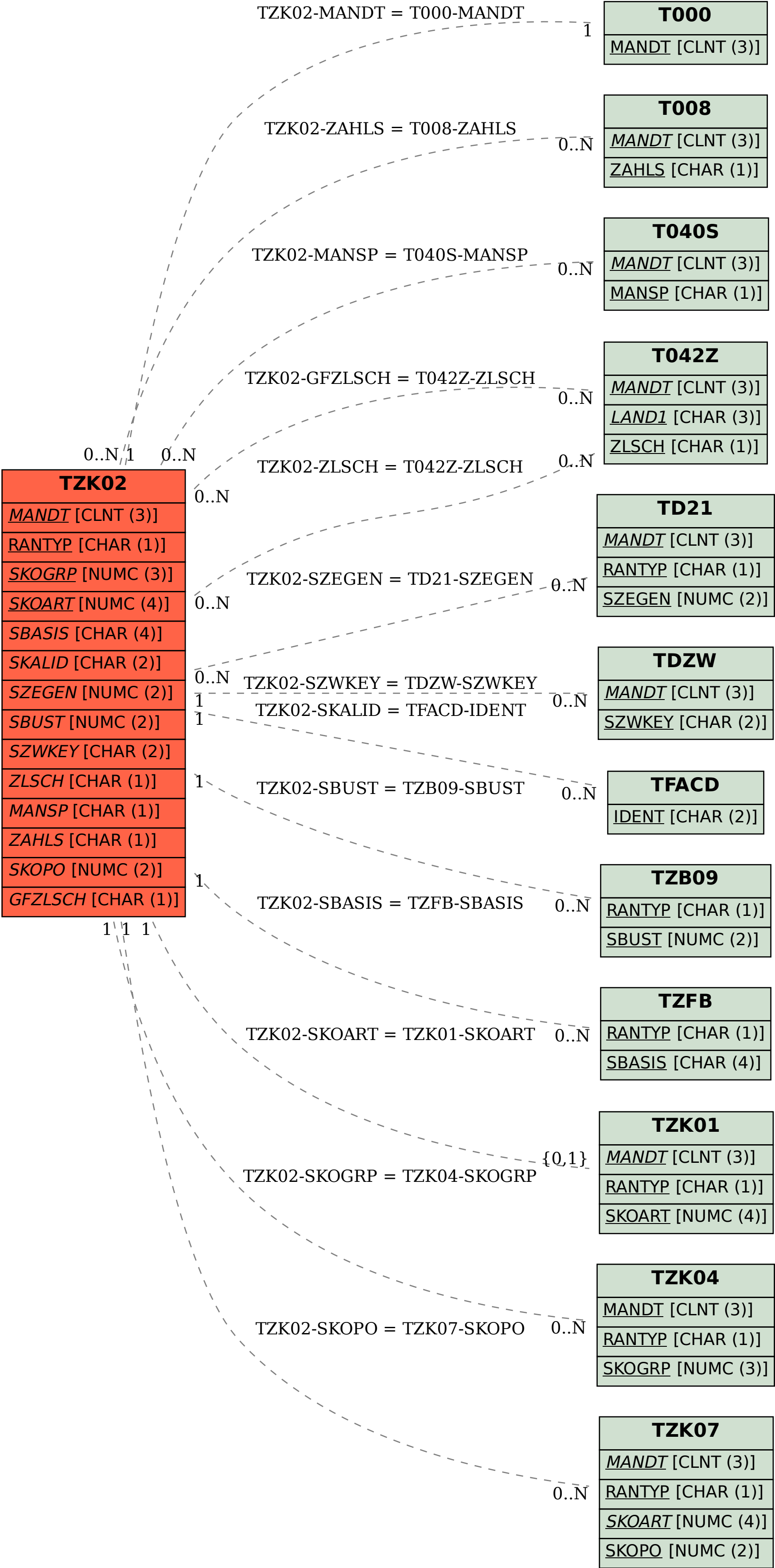
SAP ABAP table TZK02 {Condition group, condition group - condition type allocation}
