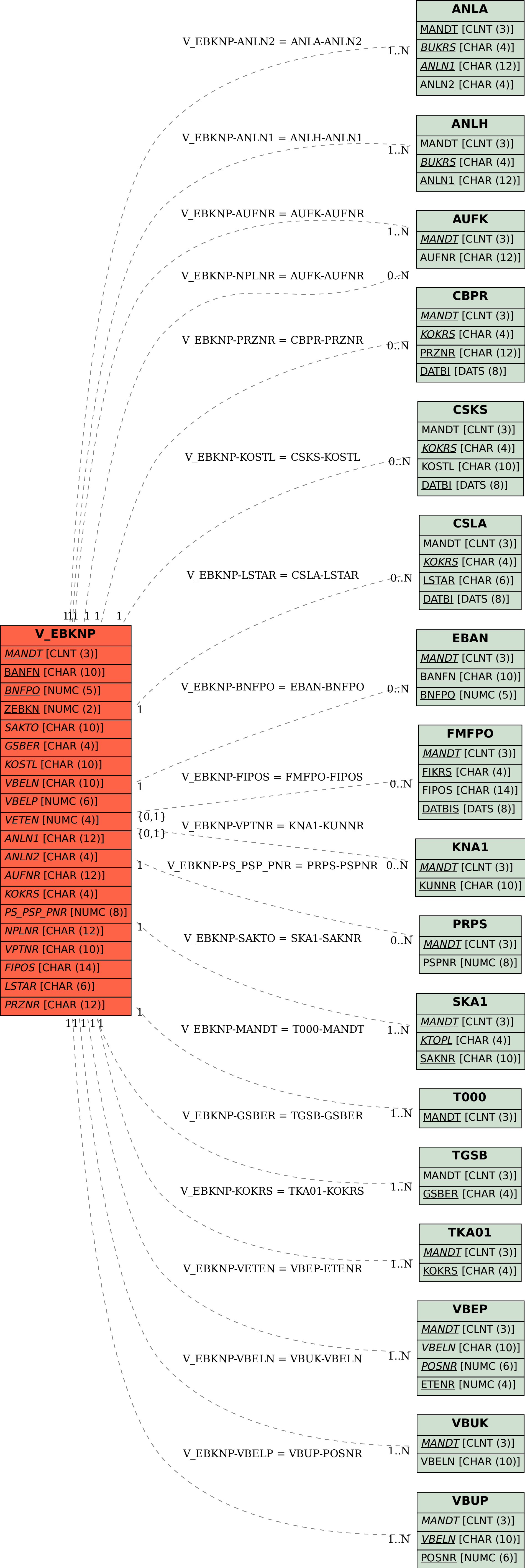
SAP ABAP table V_EBKNP {Generated Table for View}
