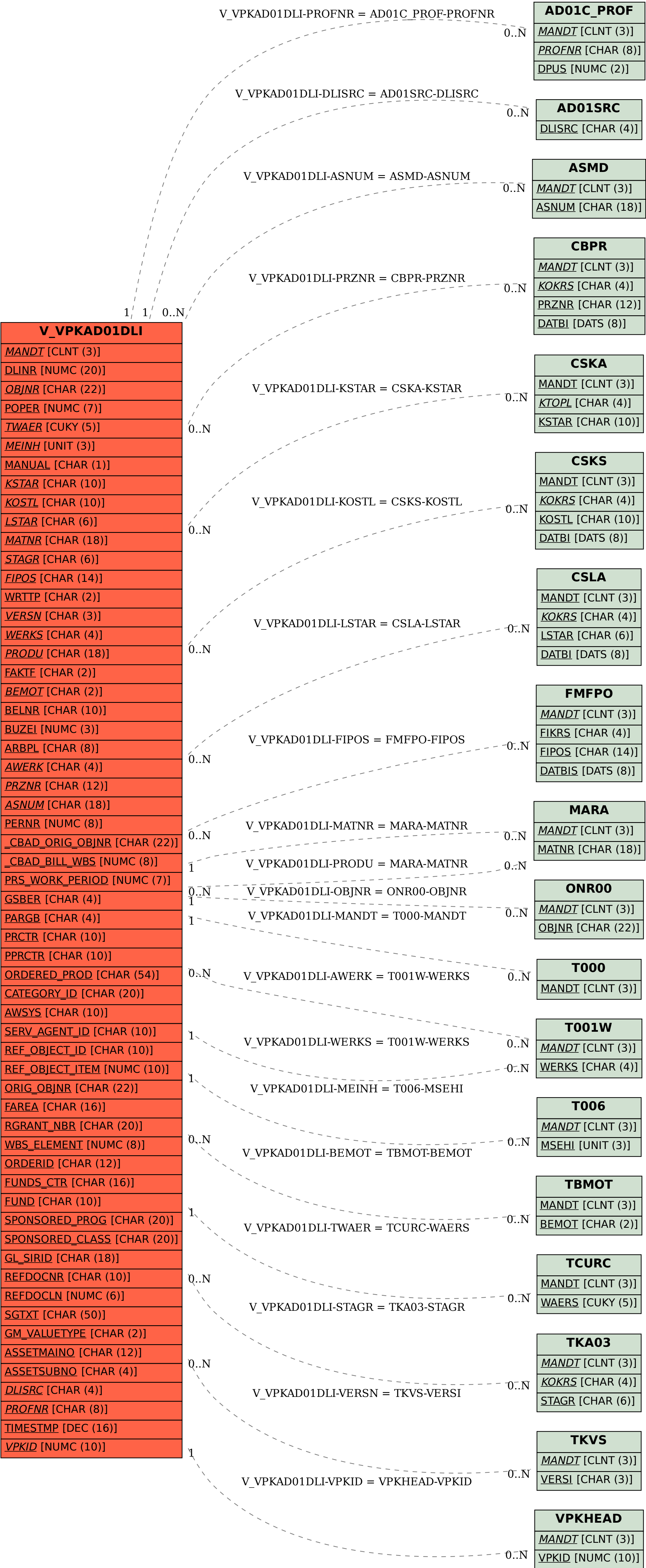
SAP ABAP table V_VPKAD01DLI {Generated Table for View}
