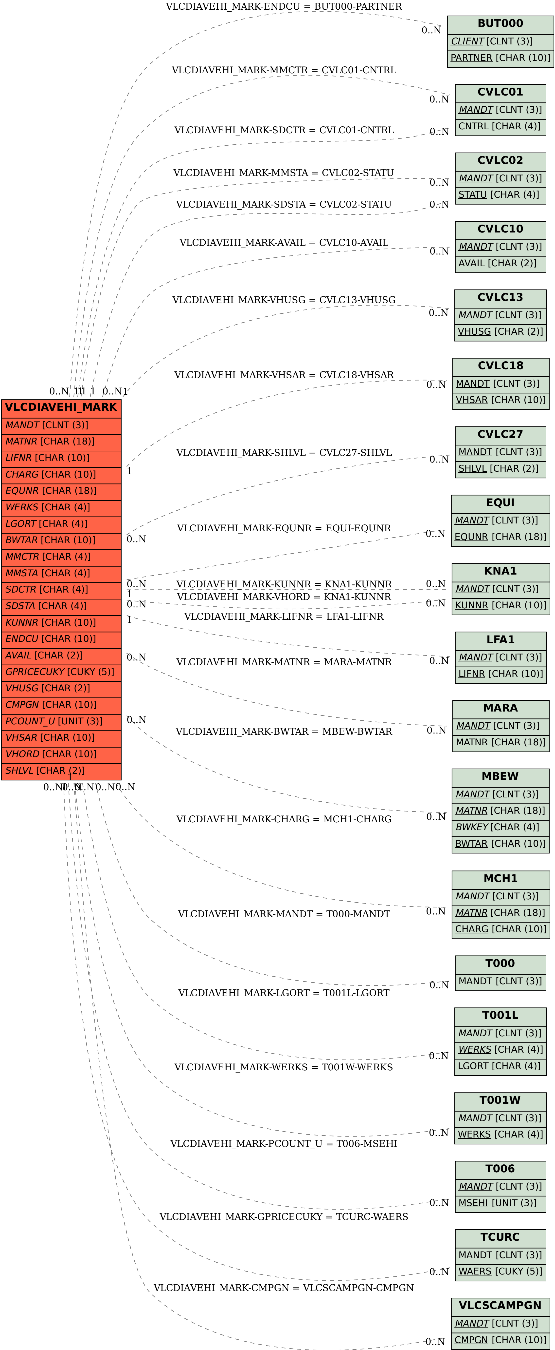
SAP ABAP table VLCDIAVEHI_MARK {VELO : Dialog Structure for Vehicles (with Selection Box)}
