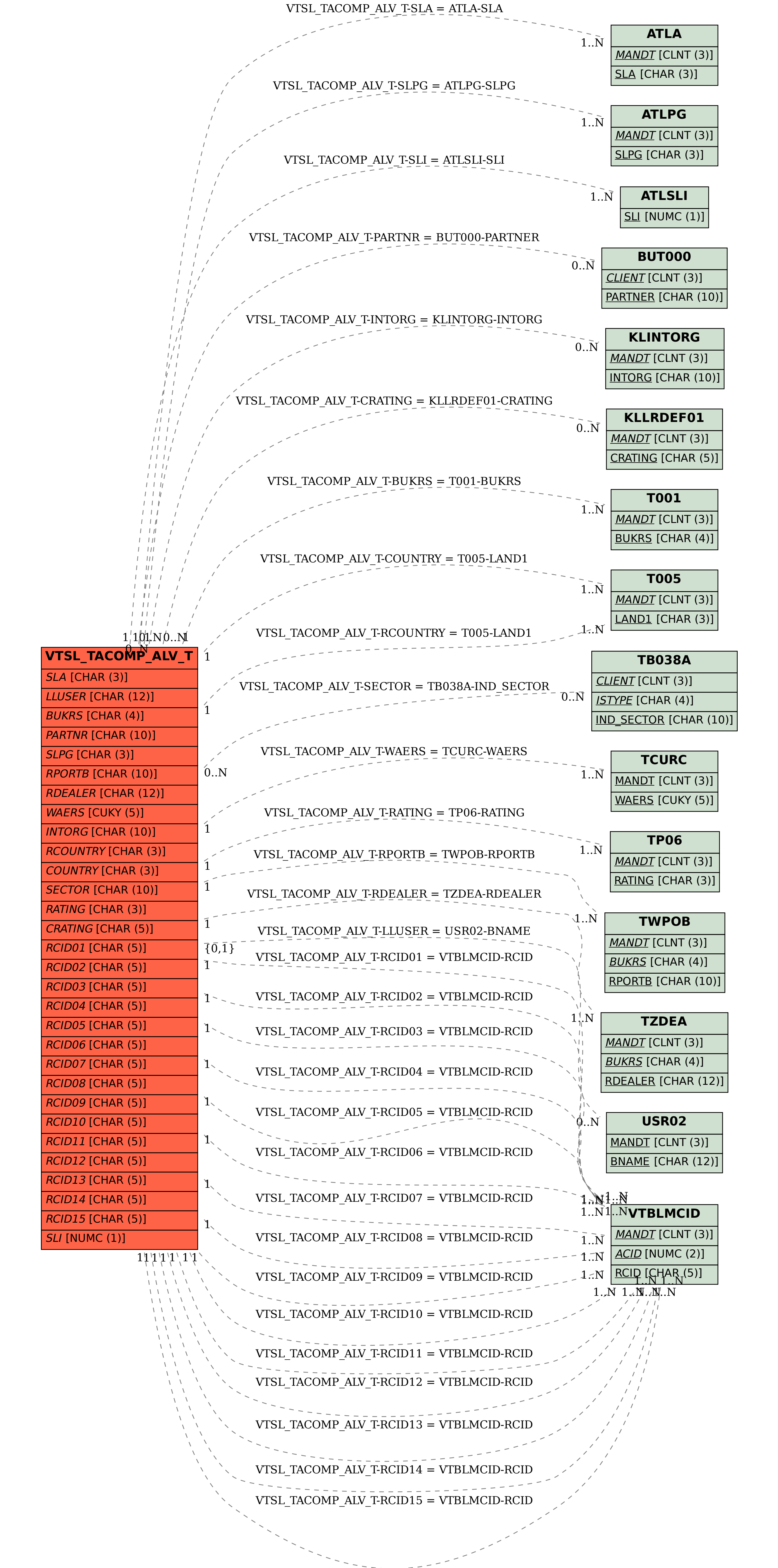
SAP ABAP table VTSL_TACOMP_ALV_T {Credit Limit: Result of Single Transaction Check for ALV}
