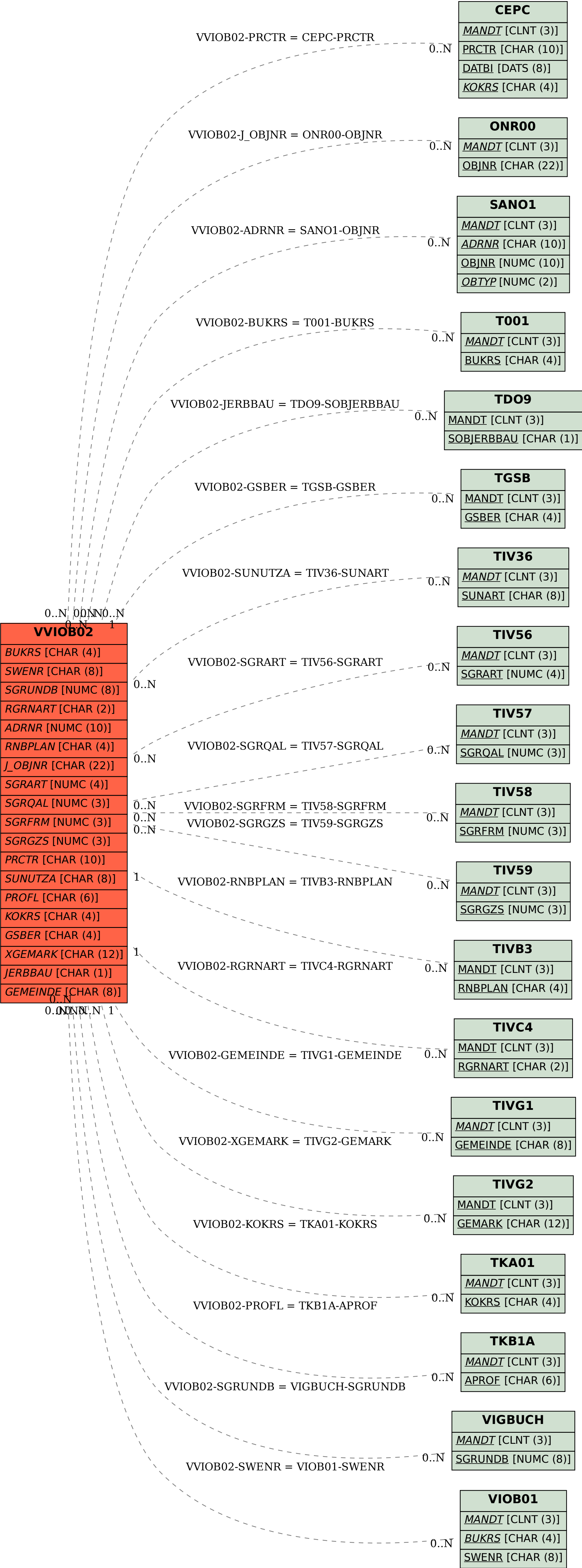
SAP ABAP table VVIOB02 {Property change structure}
