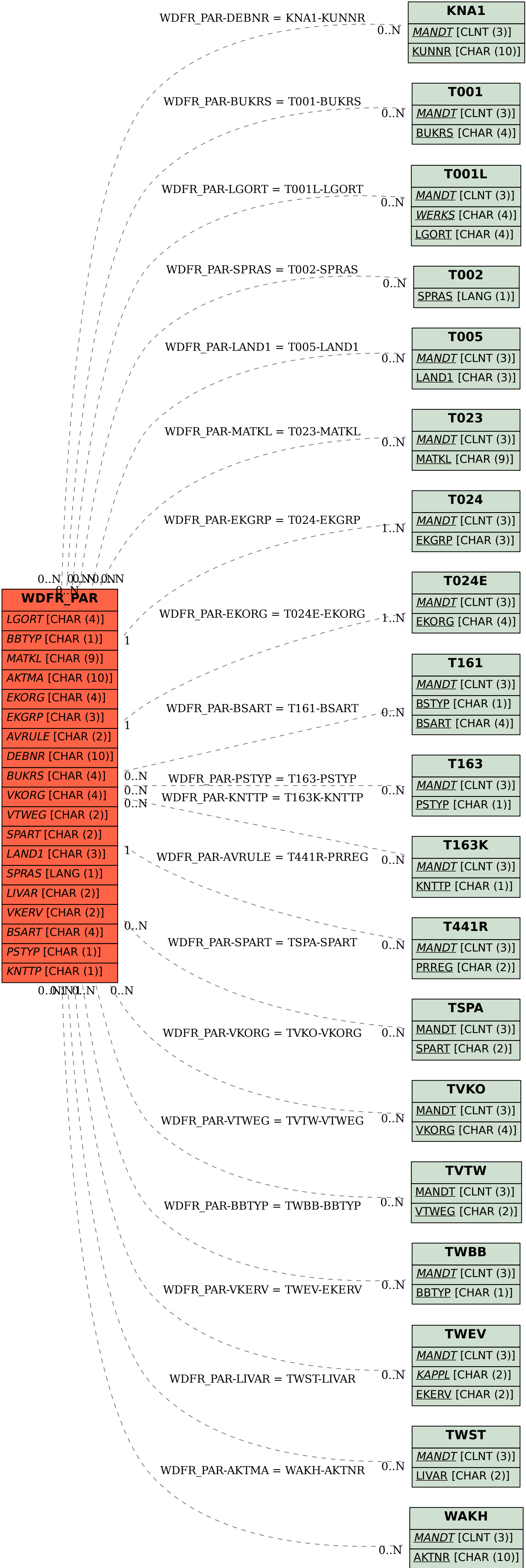
SAP ABAP table WDFR_PAR {WDFR Input Fields for Perishables Planning}
